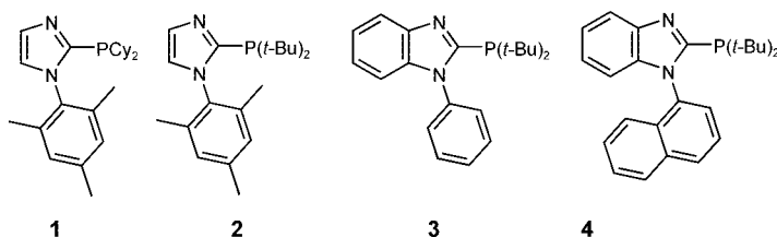
Figure 1. N -Aryl-2-(dialkylphosphino)imidazoles
